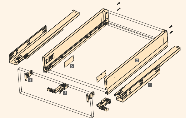
1 Opti-Motion Slide 2 Slim Panel 3 Locking Device 4 Front Connector 5 Cover Cap
