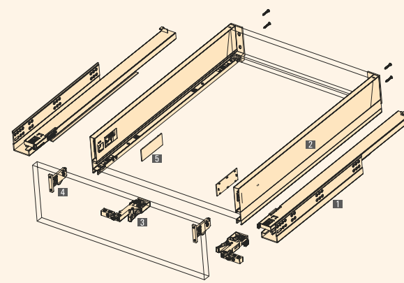
1 Opti-Motion Slide 2 Slim Panel 3 Locking Device 4 Front Connector 5 Cover Cap
