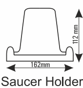
Saucer Holder
