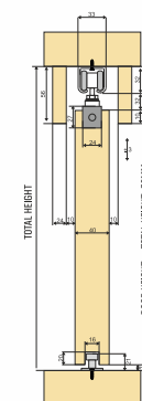
Installation Diagram
