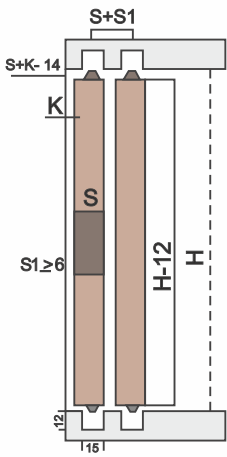
with rail end cup L=W-44
